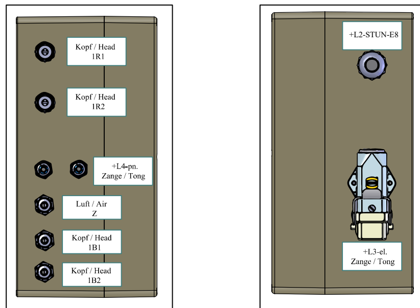
Abb. 3-23 Anschlüsse STUN-IF1-F8
