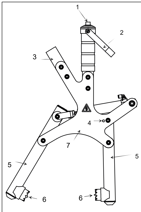
Abb. 3-20 STUN-TONG-EPP3
