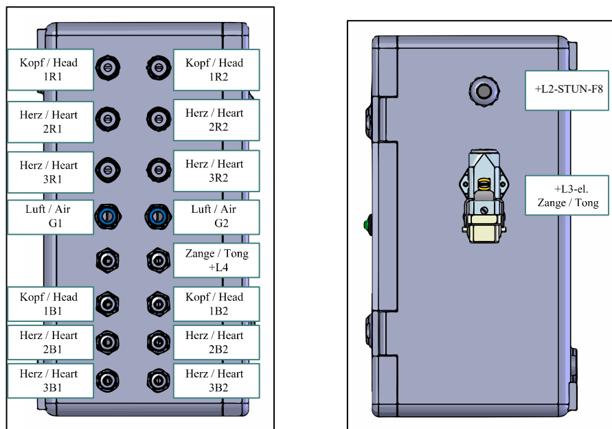
Abb. 3-24 Anschlüsse STUN-IF2-F8
