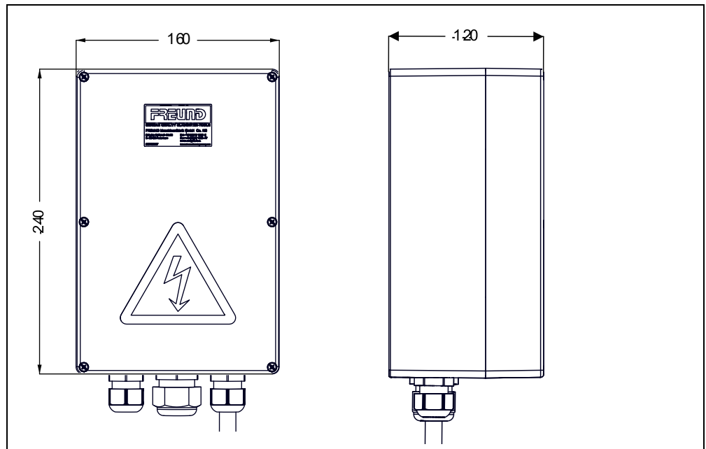
Fig. 3-10 Dimensions of the control box SG WBS51-08nc (specifications in mm)
