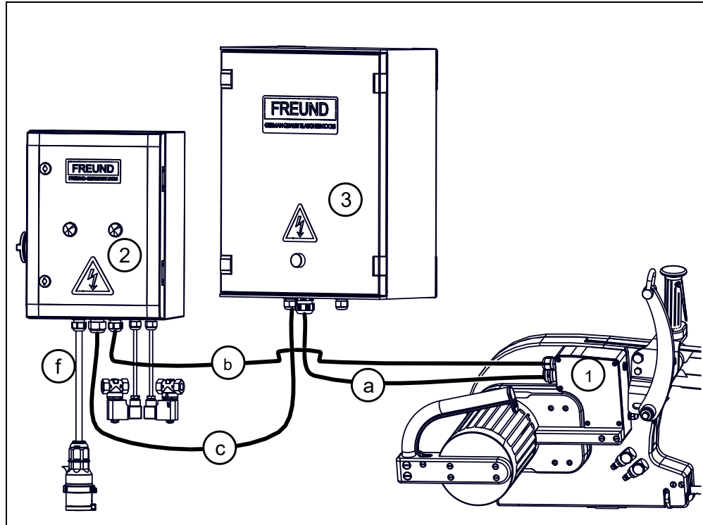
Fig. 5-6 Connection diagram
