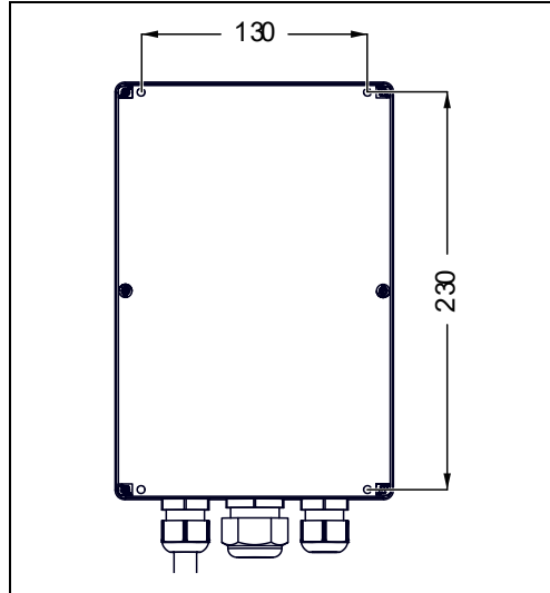
Fig. 5-4 Control box hole pattern SG WBS51-08nc [specifications in mm]
