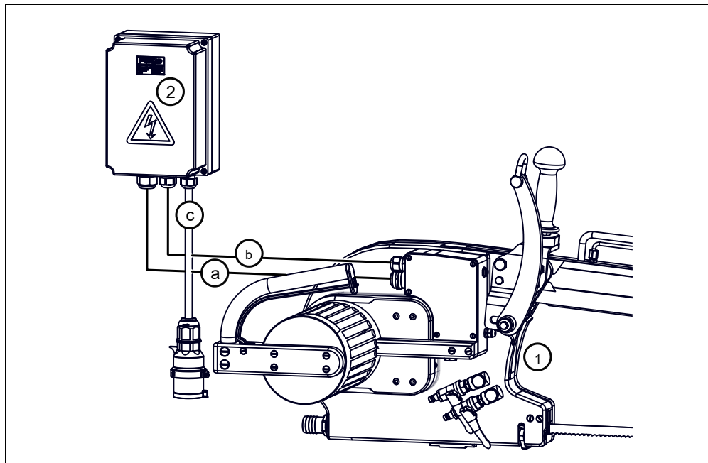
Fig. 5-9 Connection diagram
