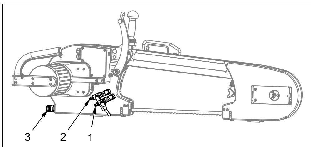
Fig. 5-10 Water connection
