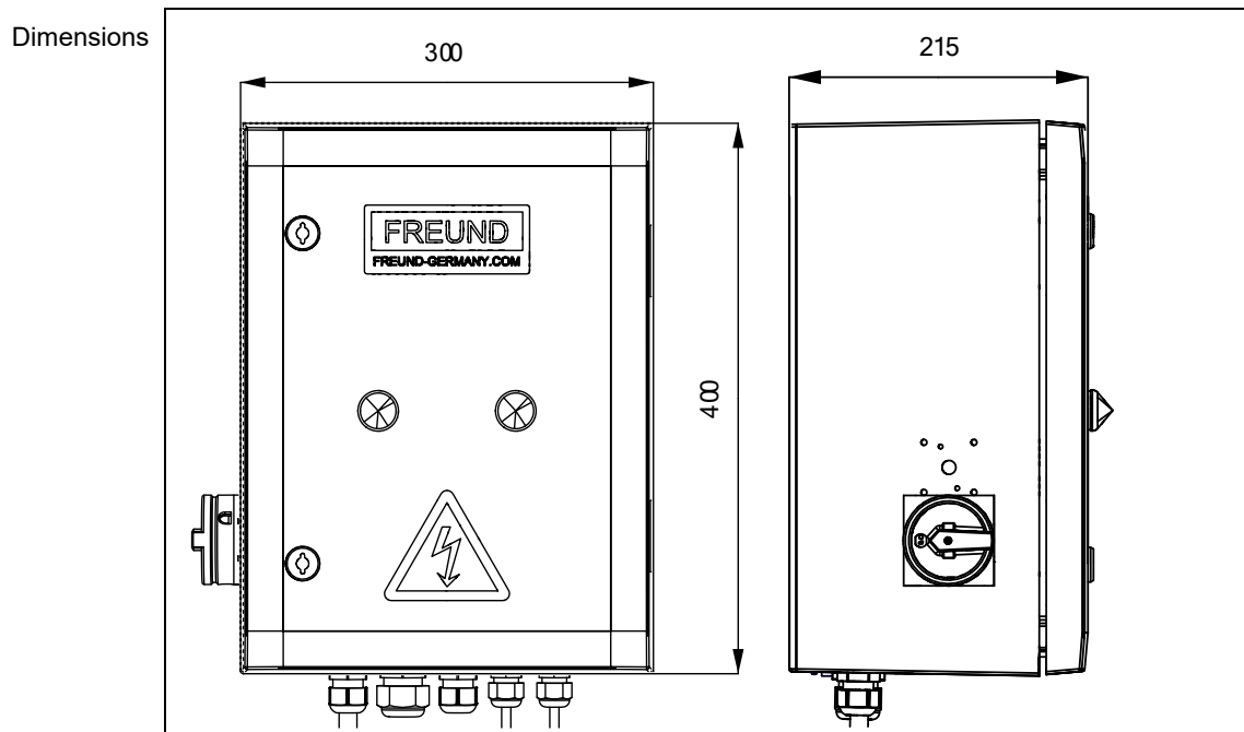
Fig. 3-8 Dimensions of the control box (specifications in mm)
