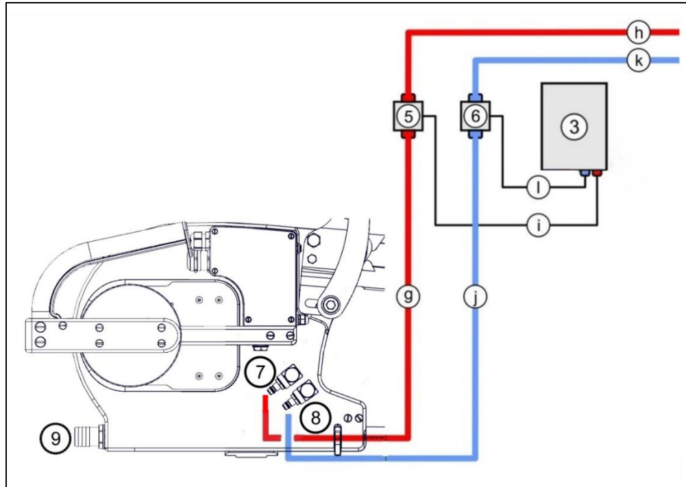
Fig. 5-8 Connection diagram
