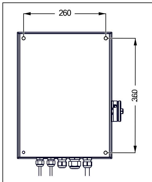
Fig. 5-2 Control box hole pattern SG WBS [specifications in mm]
