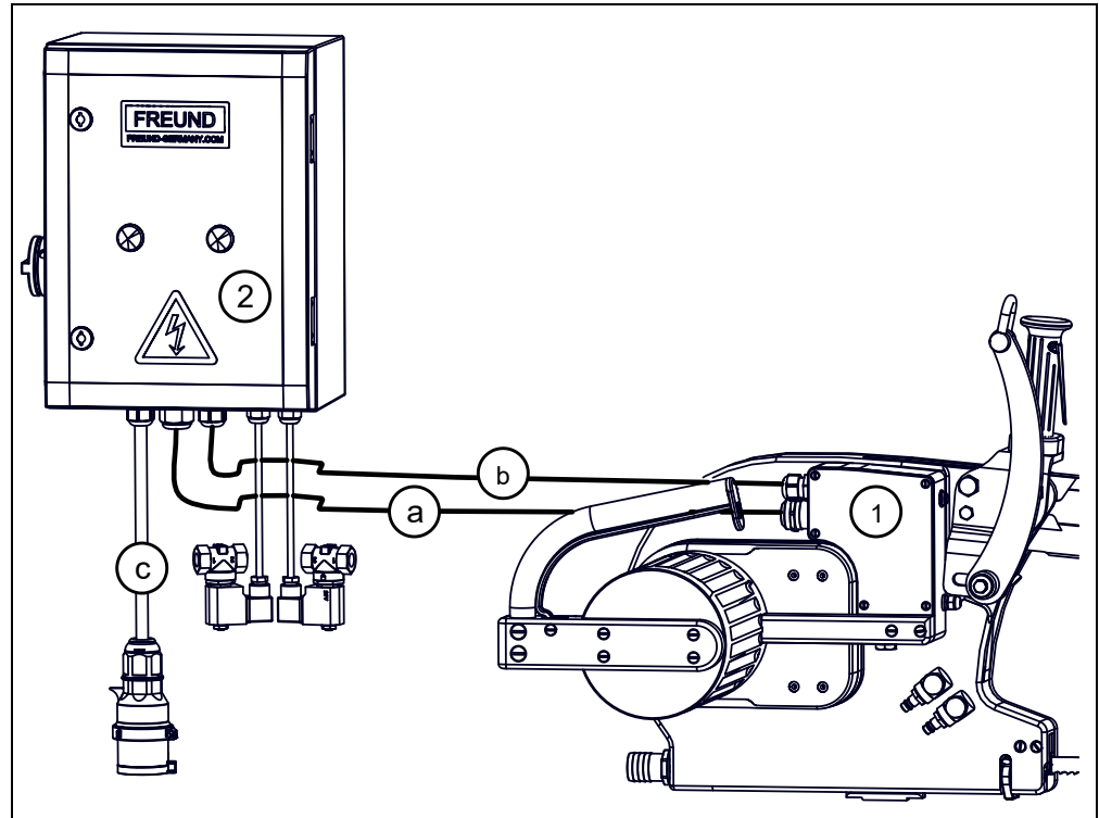
Fig. 5-7 Connection diagram
