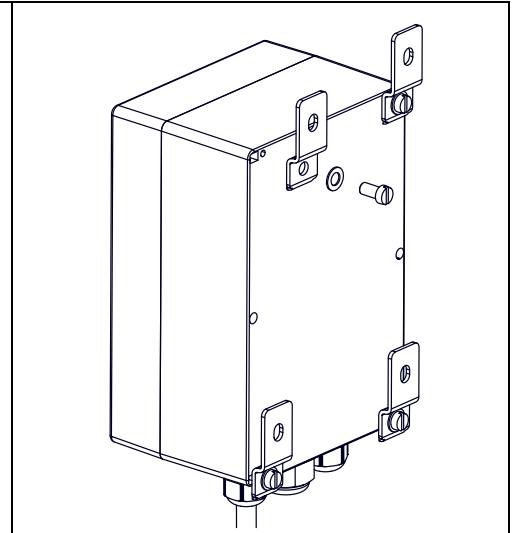
Abb. 5-5 Optionally available wall fastening set, article-no. 100-022-069
