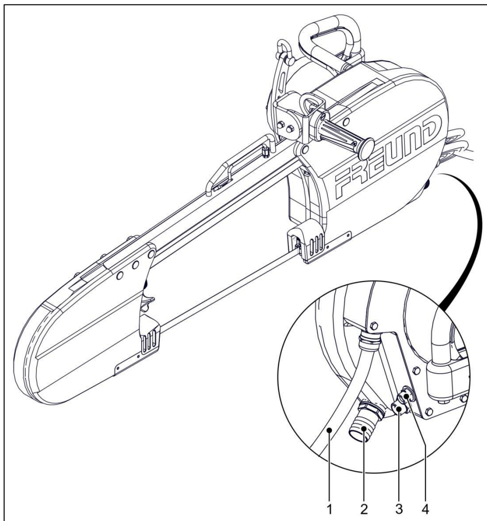
Fig. 3-2 Positions des raccordements
