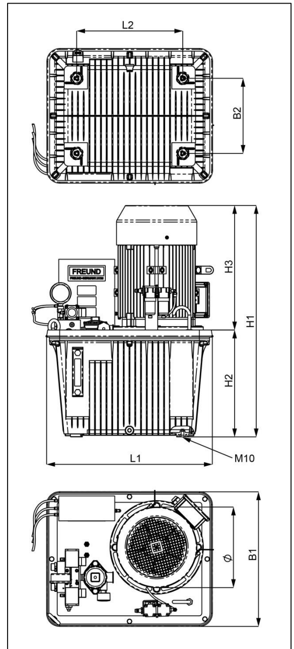
Fig. 3-10 Dimensiones HPE9/HPE20
