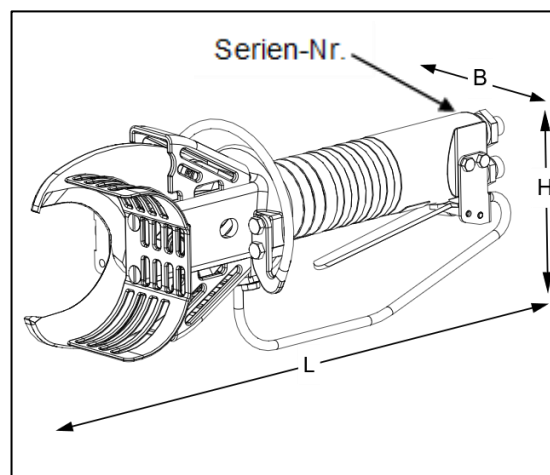
Abb. 3-2 Schere Model FS6
