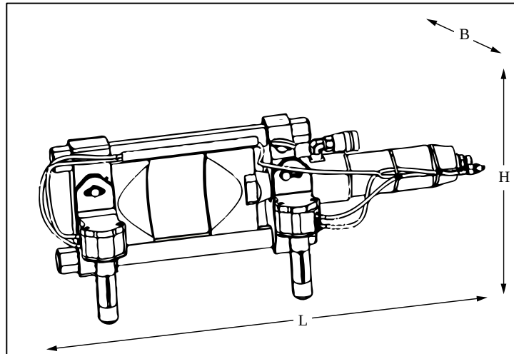
Abb. 3-12 Hornguillotine HG12 evo2
