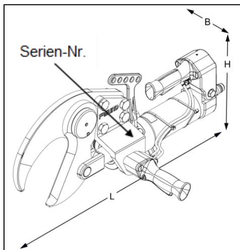
Abb. 3-6 Schere Model HLS12
