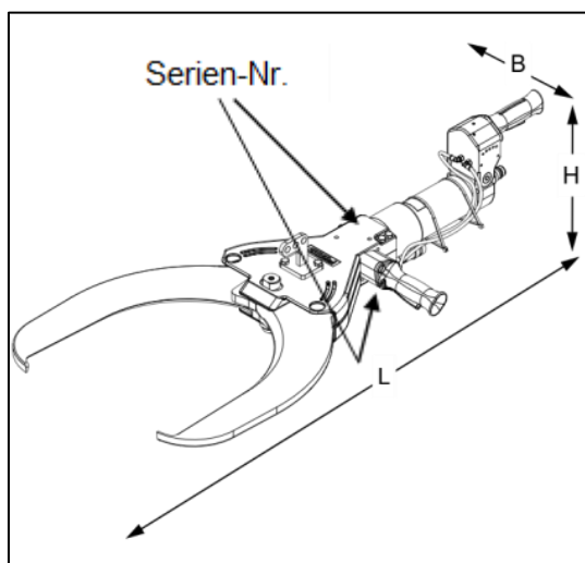
Abb. 3-11 Schere Model AS28
