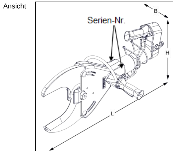
Abb. 3-7 Schere Model LS15
