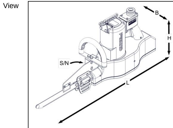
Fig. 3-2 Example of reciprocating breastbone saw
