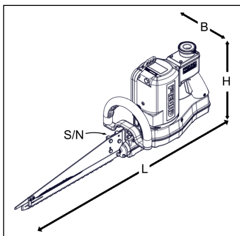
Fig. 3-6 Example of reciprocating breaking saw
