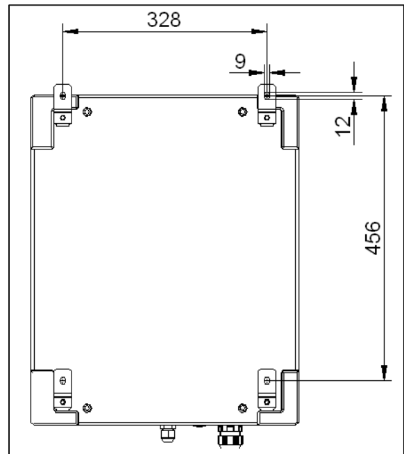
Fig. 5-2 Drill pattern
