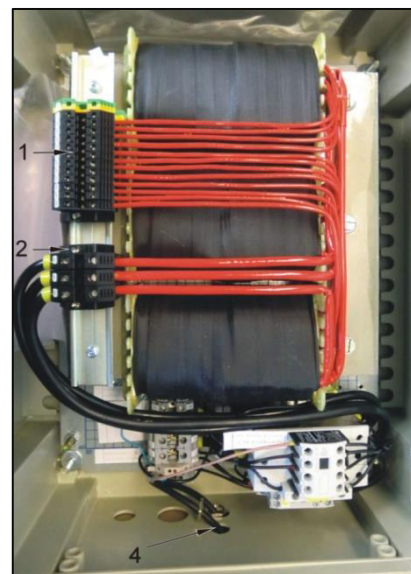
Fig. 5-9 Connections inside TR7
