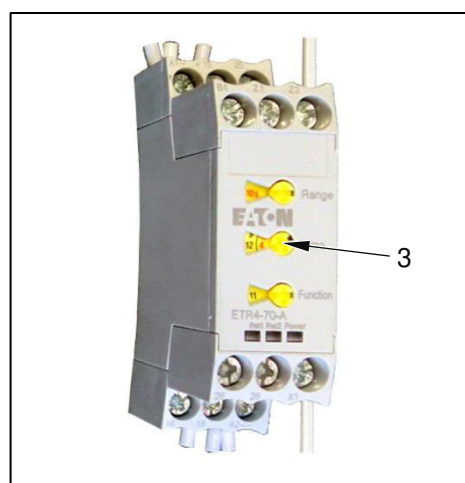
Fig. 3-12 Time-lag relay
