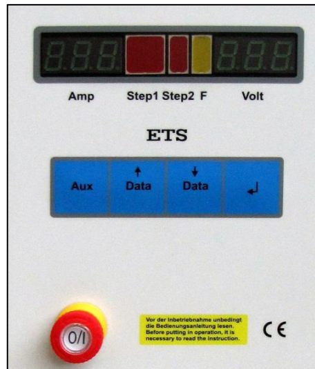
Fig. 3-18 Control and display panel
