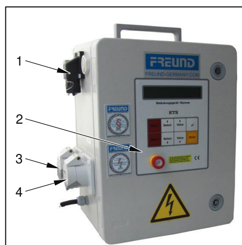
Fig. 3-3 Function elements
