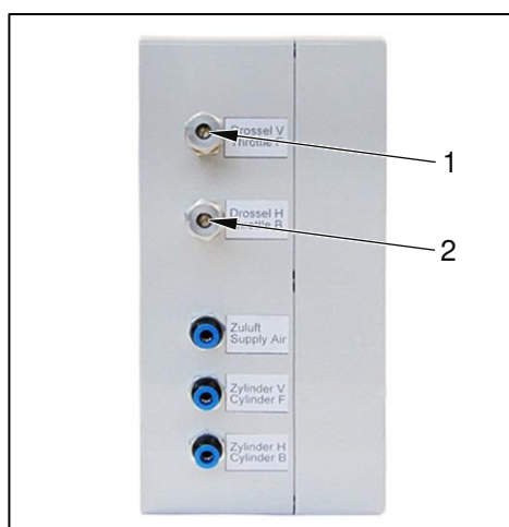
Fig. 3-11 Throttle valve
