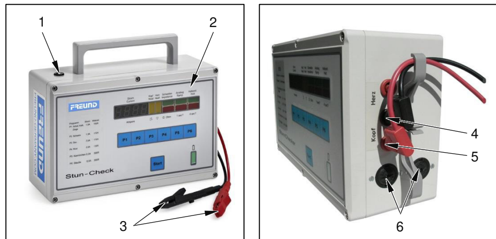
Fig. 3-15 Function elements
