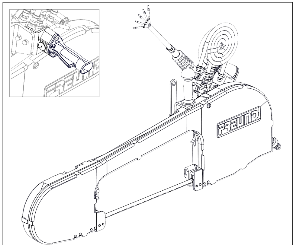
Fig. 3-2 View of standard machine SB49-08, detail: SB549-08 with 2HATD
