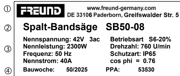
Fig. 3-4 Example of rating plate on front of motor
