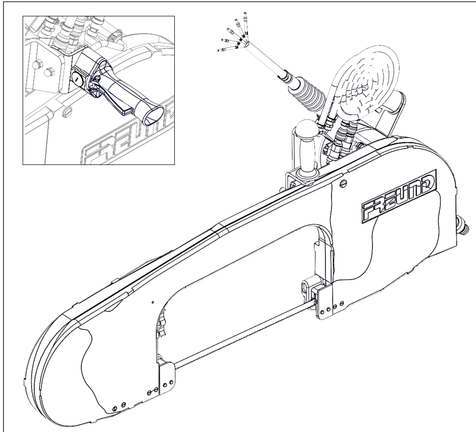
Fig. 3-1 View of standard machine SB46-08, detail: SB46-08 with 2HATD
