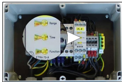
Fig. 5-5 Timer relay in control box
