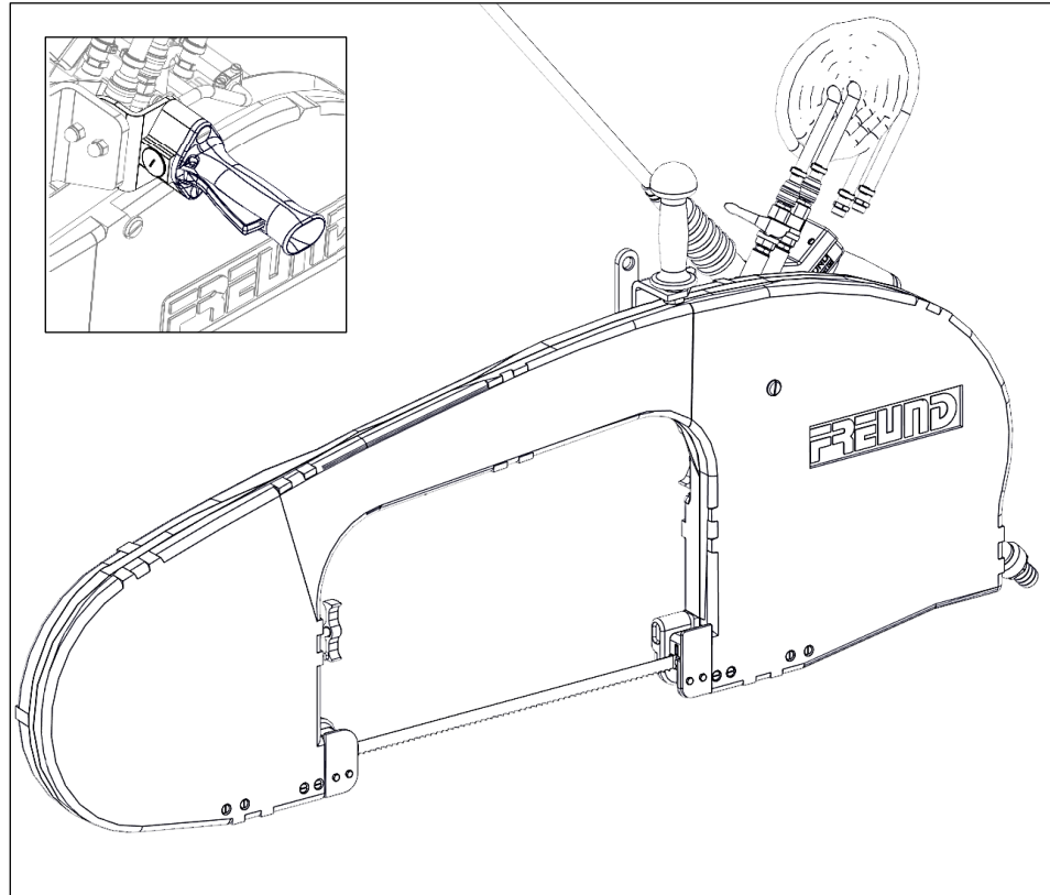
Fig. 3-3 View of standard machine SB50-08, detail: SB50-08 with 2HATD
