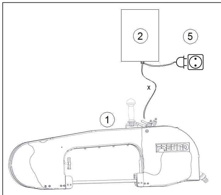
Fig. 5-1 Connection diagram for 42 V machines
