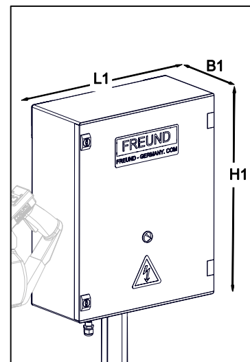
Fig. 3-7 Illustration example for control box
