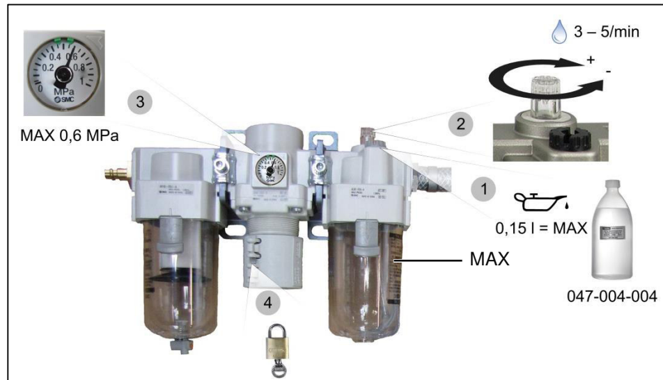
Fig. 5-21 Connecting the service unit
