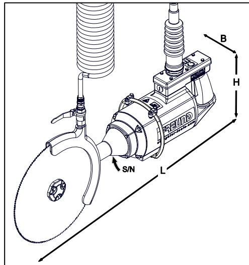
Fig. 3-5 Illustration example for circular splitting saw SK32 and SK40 (S/N = serial number)
