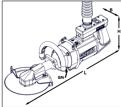
Fig. 3-10 Illustration example for circular bacon saws
