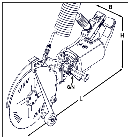
Fig. 3-6 Illustration example for circular splitting saw with motor 08 (S/N = serial number)
