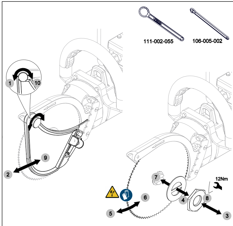
Fig. 8-1 Changing the saw blade (example: K18-01)
