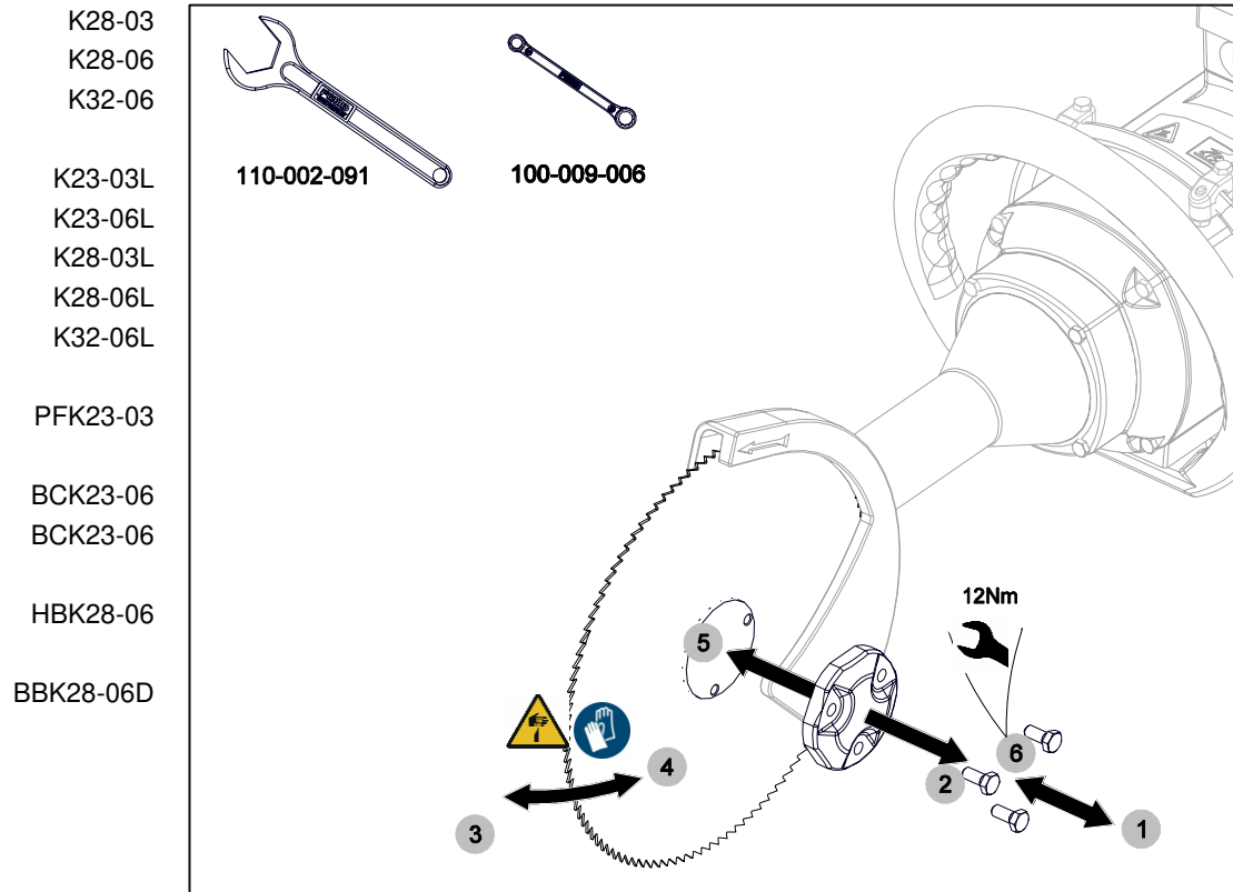
Fig. 8-3 Changing the saw blade (example: K23-06L)
