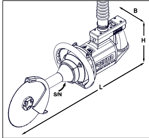
Fig. 3-14 Illustration example for circular breaking and quartering saws
