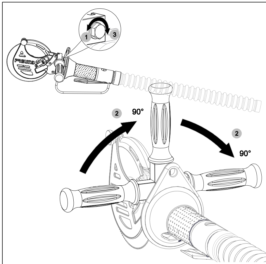
Fig. 5-22 Possible handle positions
