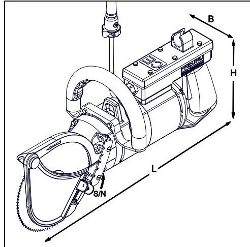
Fig. 3-11 Illustration example for alternating current circular breaking saws
