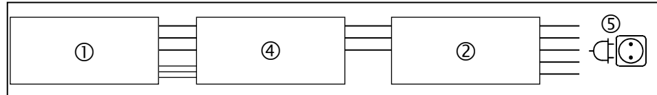
Fig. 5-8 Connecting lines for machines with 2HADTS
