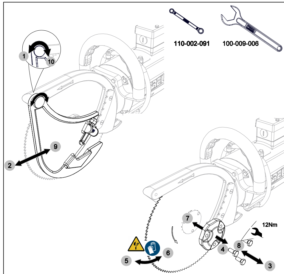
Fig. 8-2 Changing the saw blade (example: K23-03)
