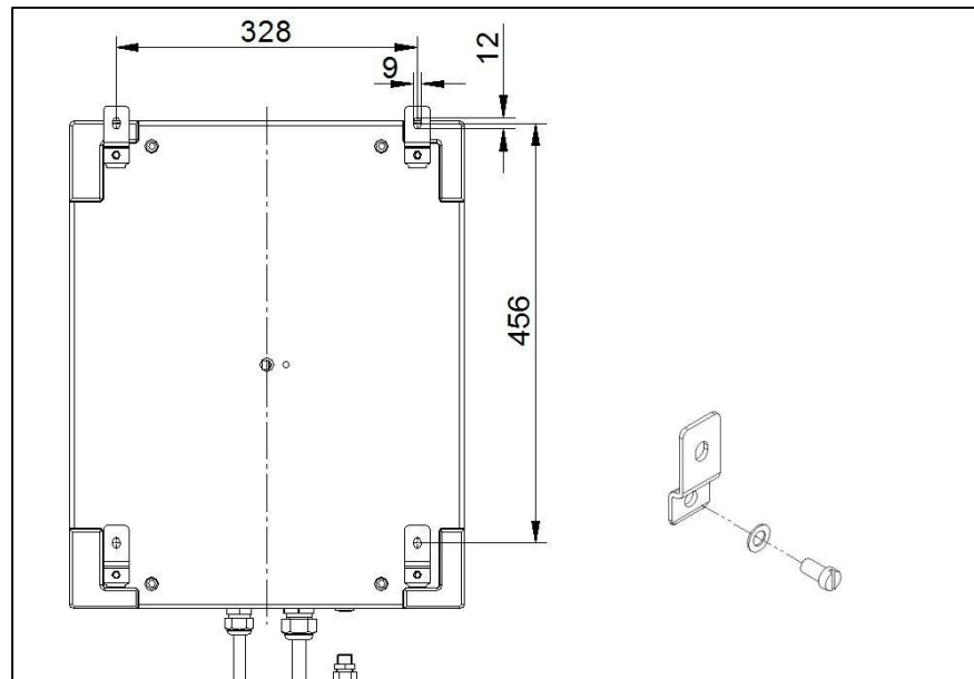
Fig. 5-13 Control box hole pattern 2HATDS/EMBS and wall fastening set
