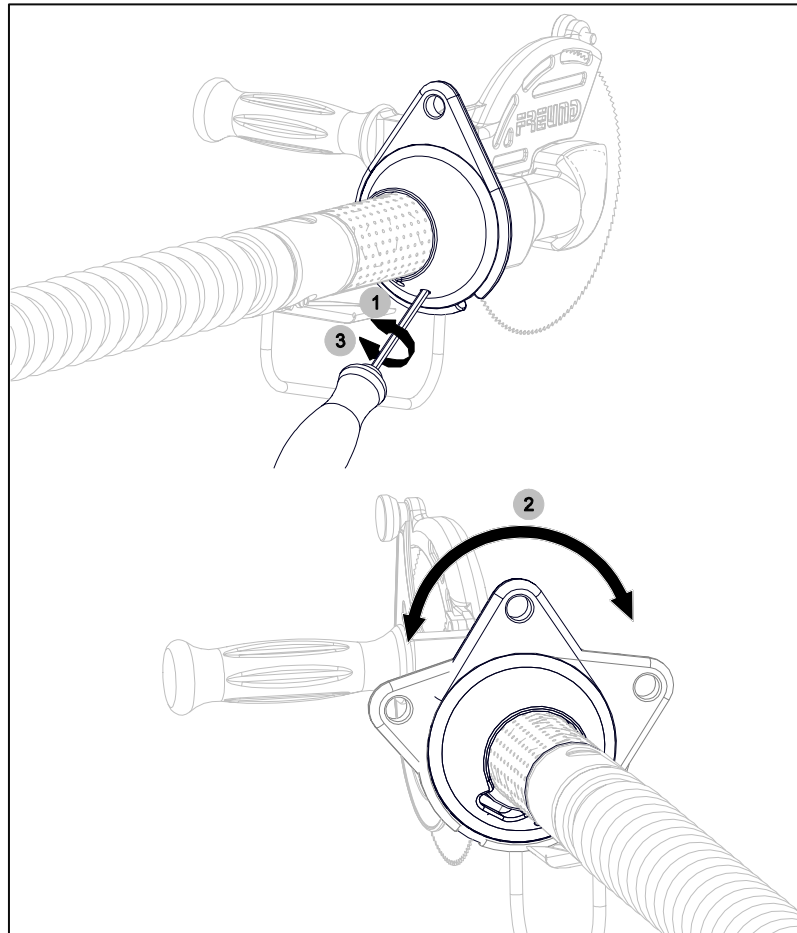
Fig. 5-23 Possible hanger positions
