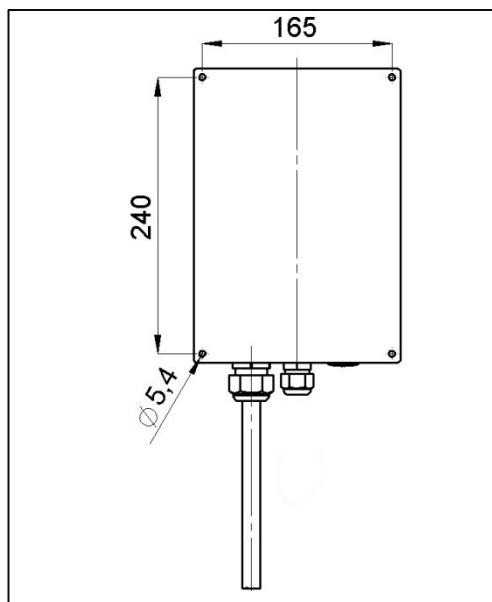
Fig. 5-6 Control box hole pattern 2HATDS 42V
