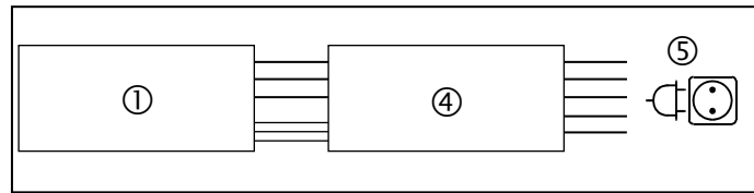
Fig. 5-16 Connecting lines for machines with 2HADTS
