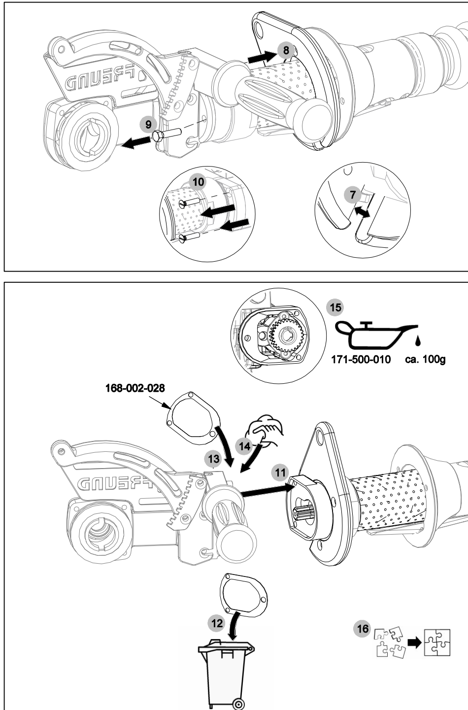
Fig. 8-9 Work steps for greasing the intermediate gear unit for K16-P4_evo2
