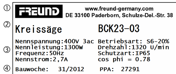
Fig. 3-1 Rating plate example
