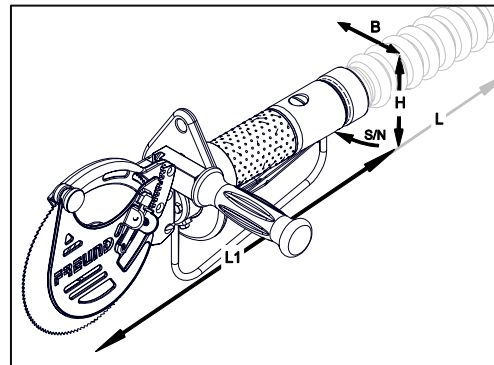
Fig. 3-8 Illustration example for pneumatic circular breaking saw
