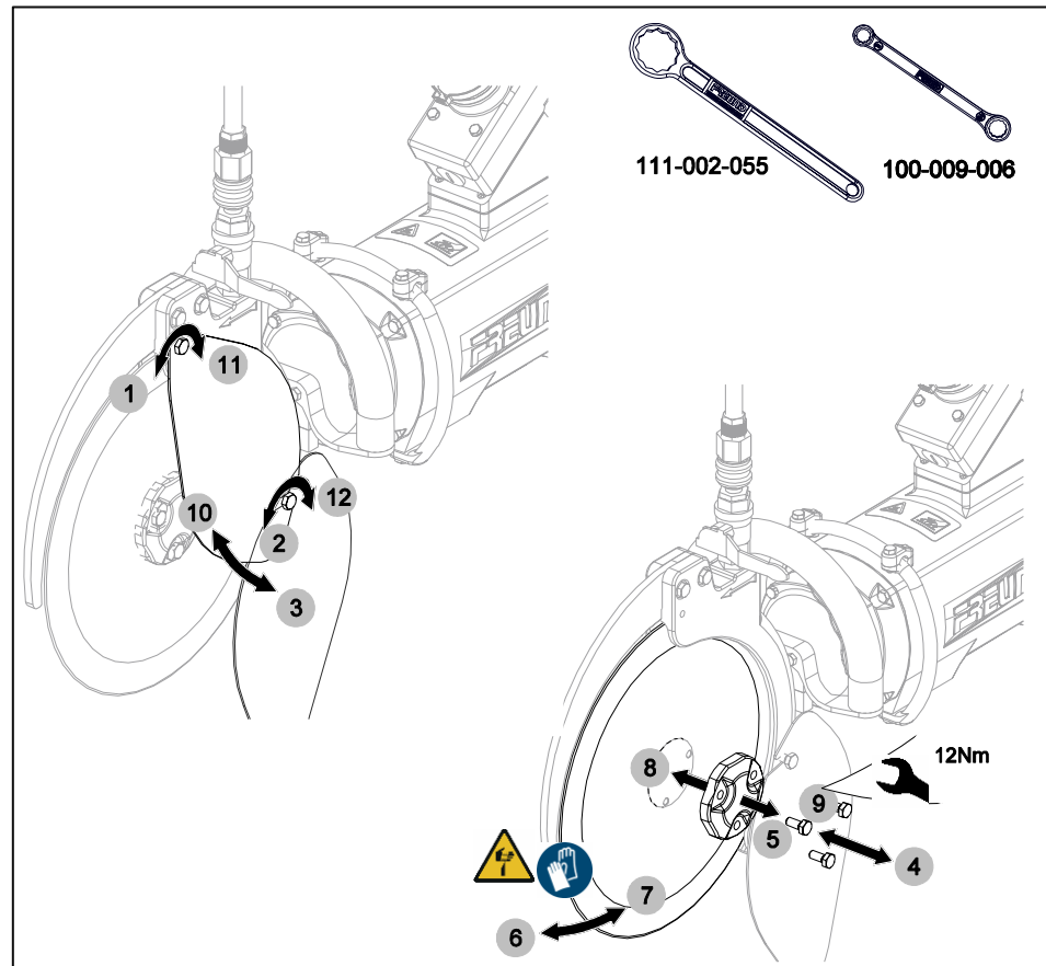
Fig. 8-5 Replacing the circular blade BBKM25
