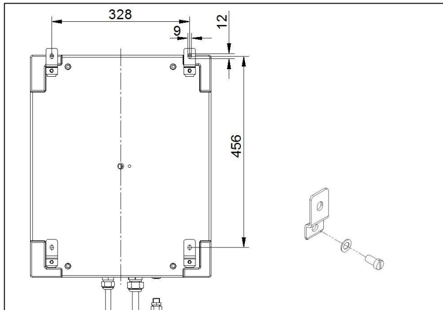
Fig. 5-5 Control box hole pattern 2HATDS/EMBS and wall fastening set
