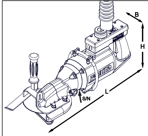
Fig. 3-9 Illustration example for the riptop circular saw
