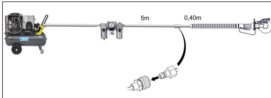
Fig. 5-19 Connection diagram for machine K16-P4_evo2
