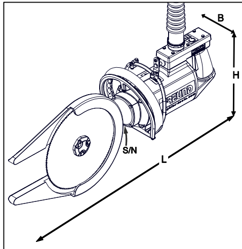
Fig. 3-2 Illustration example for circular horn and leg saws (S/N = serial number)
