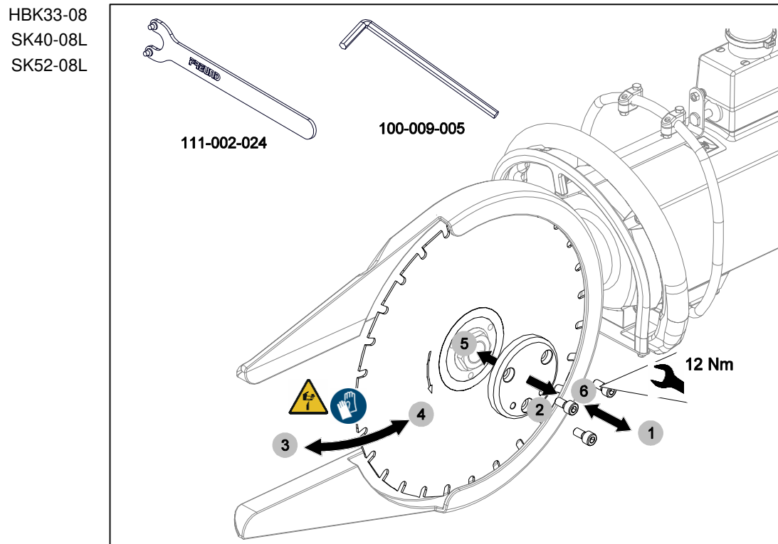
Fig. 8-4 Changing the saw blade (example: HBK33-08)
