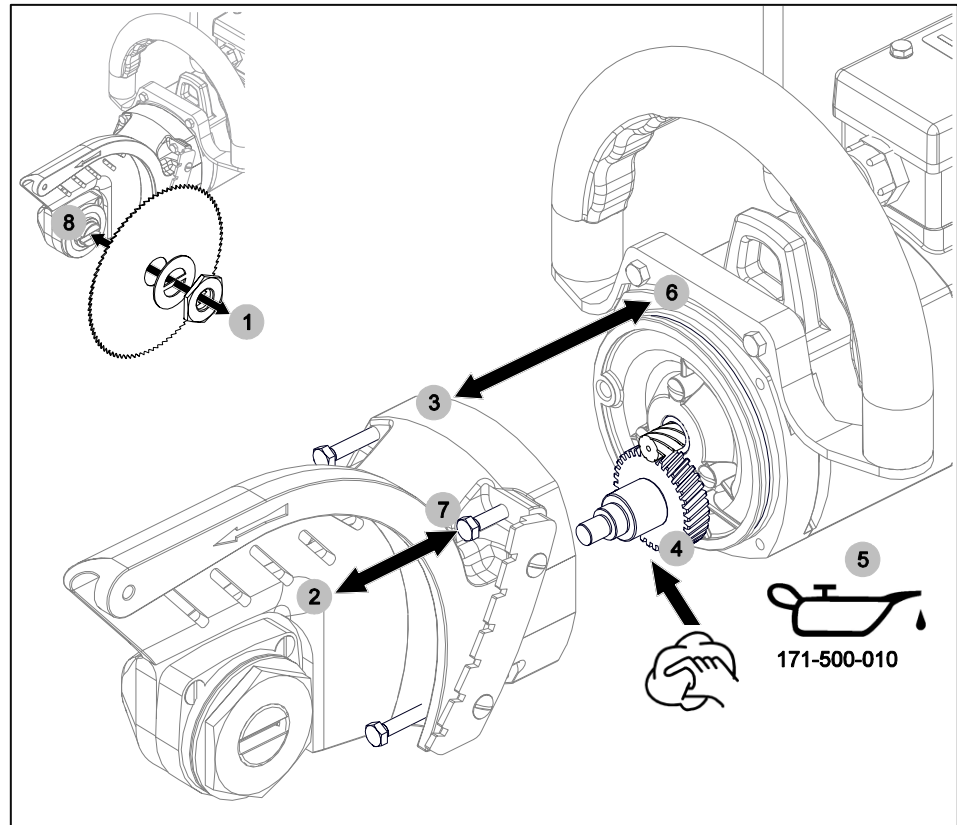
Fig. 8-7 Work steps for greasing the intermediate gear unit K18 01
