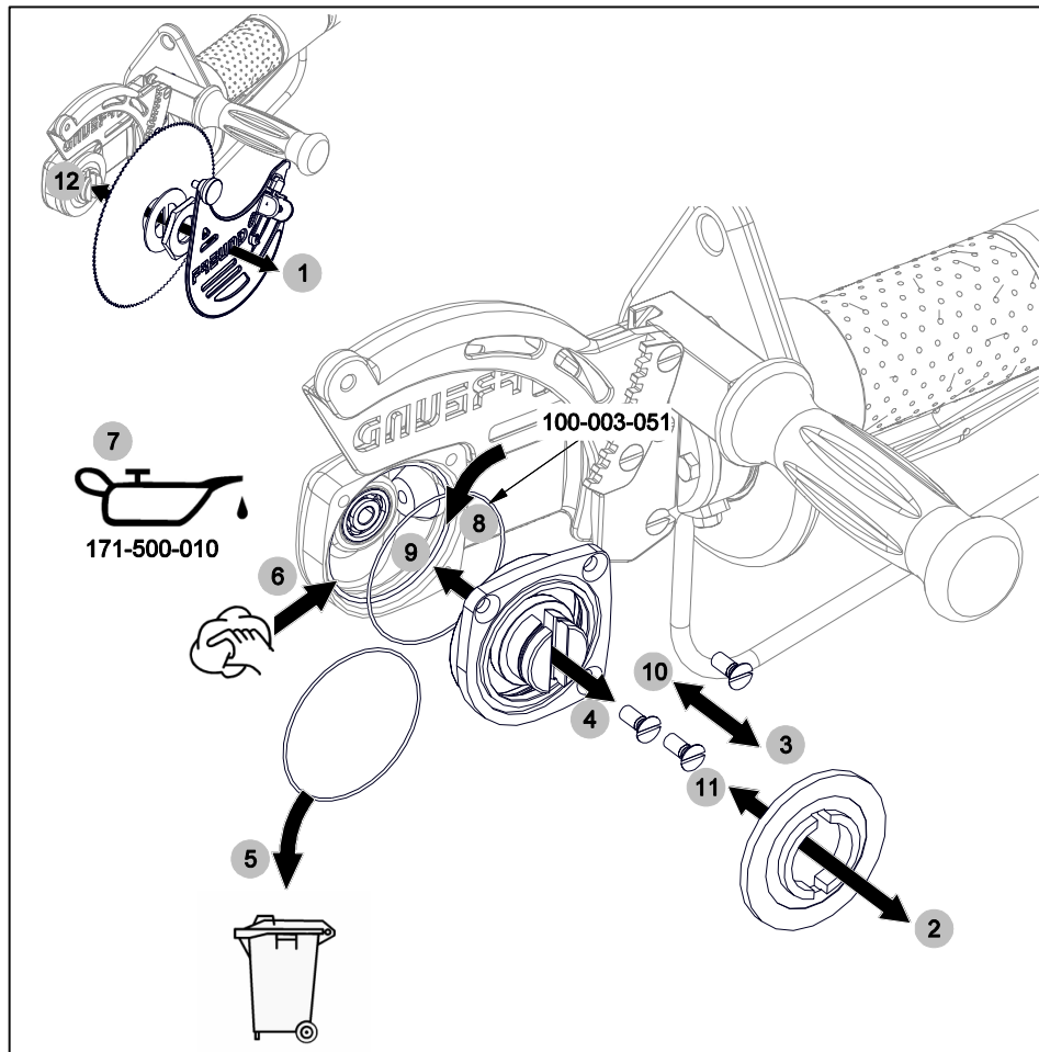
Fig. 8-8 Work steps for greasing the bevel gear unit for K16-P4_evo2
