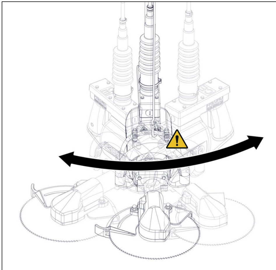
Fig. 6-1 Rotary movement on switching on the machine, example for BCK23-03
