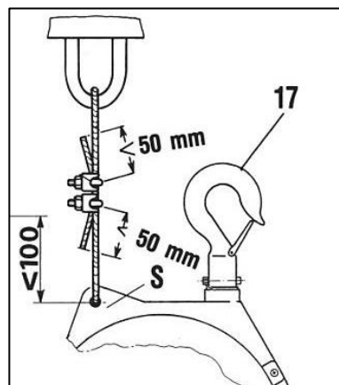
Fig. 4-1 Drop height
