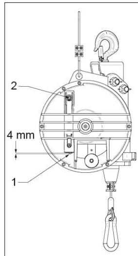
Fig. 5-3 Clamping screw
