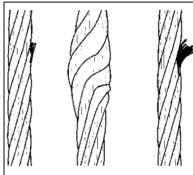
Fig. 6-1 Visible damage to the cable
