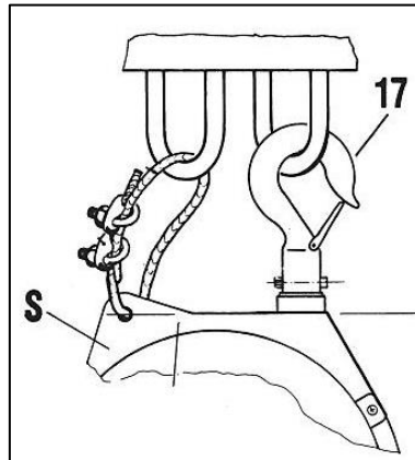
Fig. 4-3 Safety suspension
