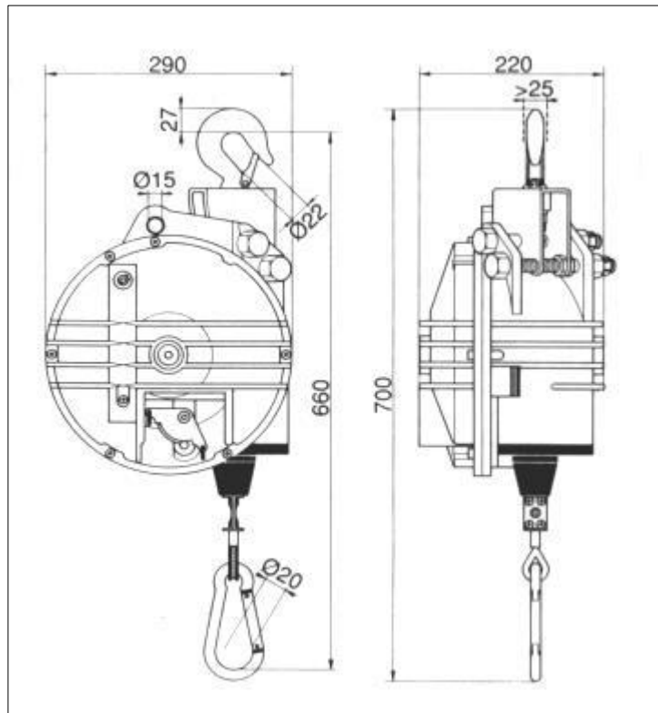
Fig.3-1 Dimensions of balancers F20-F35
