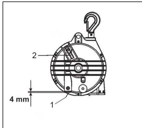
Fig. 5-3 Clamping screw
