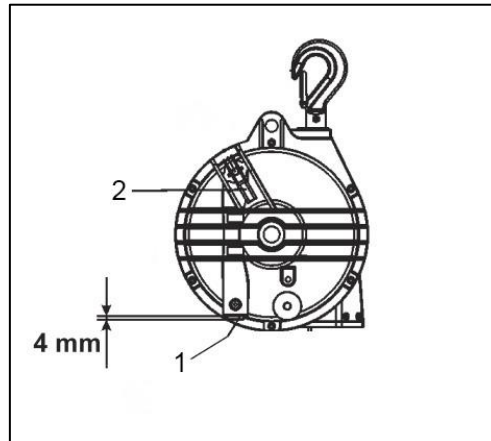
Fig. 5-3 Clamping screw
