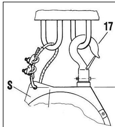
Fig. 4-3 Safety suspension
