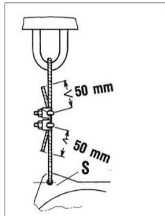
Fig. 4-4 Fitting the safety cable
