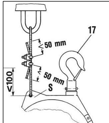
Fig. 4-1 Drop height
