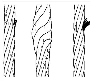
Fig. 6-1 Visible damage to the cable
