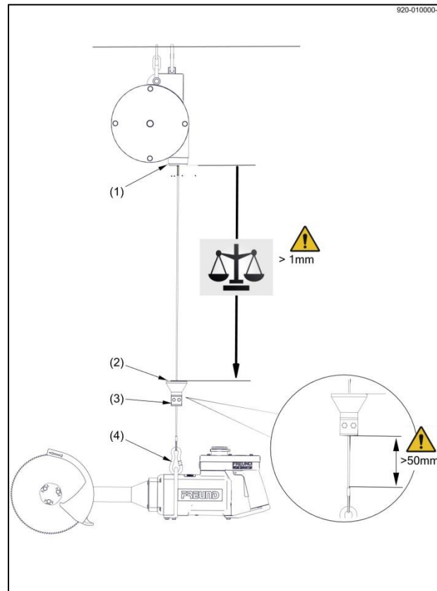
Fig. 5-1 Attached circular saw
