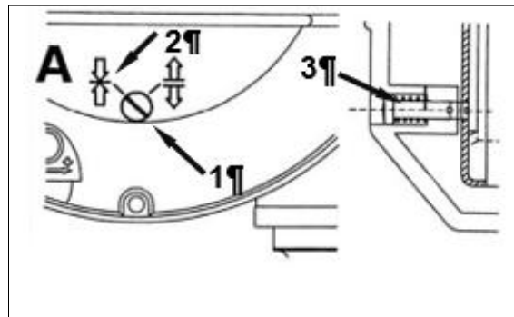
Fig. 5-4 Blocking the drum
