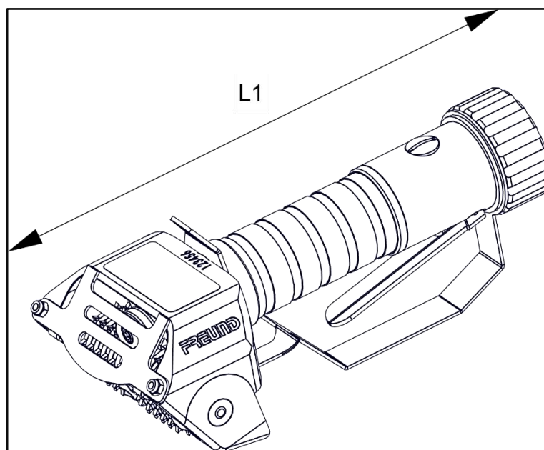
Ilust. 3-1 Hand-Skinner HSK8-P5 montado
