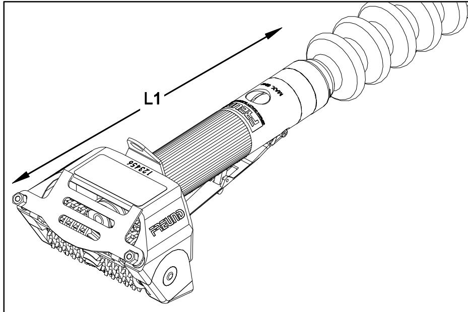
Ilust. 3-3 Hand-Skinner HSK8-P3 montado
