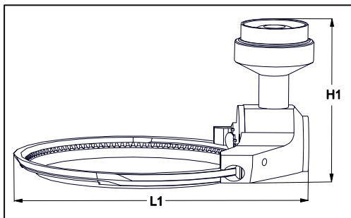
Fig.3-1 Side view
