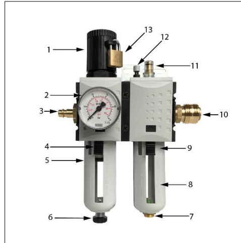
Fig. 3-7 Service unit
